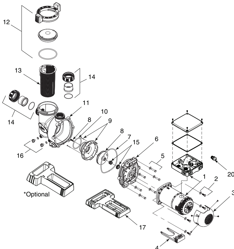
Figure 16. Jandy Variable Speed Pump Exploded View (Specific models may differ slightly from illustration)
