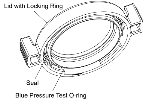
Figure 11. Blue Pressure Test O-Ring
