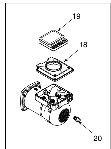
Motor/Drive Exploded View (Pump Models Ending in DVS)
